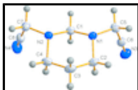
Fig. 1. A view of the title molecule. Displacement ellipsoids are drawn at the 50% probability level.
