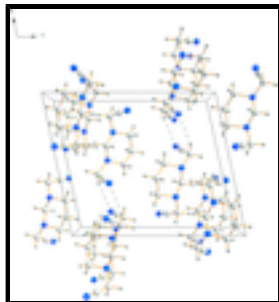
Fig. 2. Packing of the molecules of the title compound view along the b axis. Dashed lines represent intermolecular hydrogen bonds.
